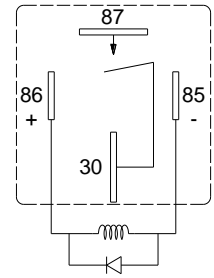
With Parallel Diode (Anode on 85#)
