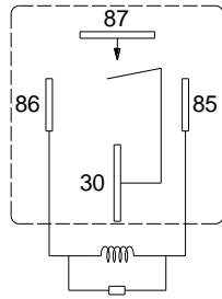
With Resistor
