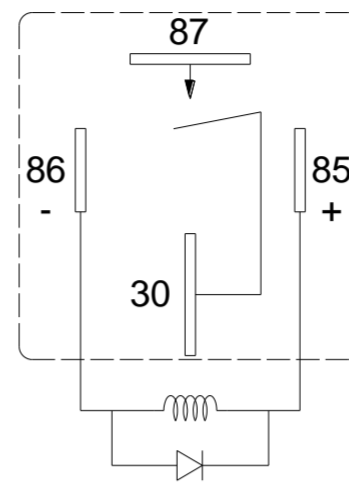
With Parallel Diode (Anode on 86#)
