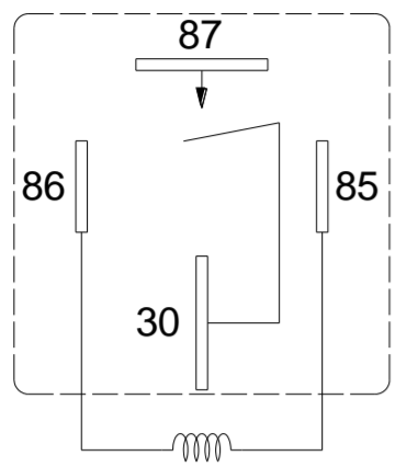
Without Parallel Components
