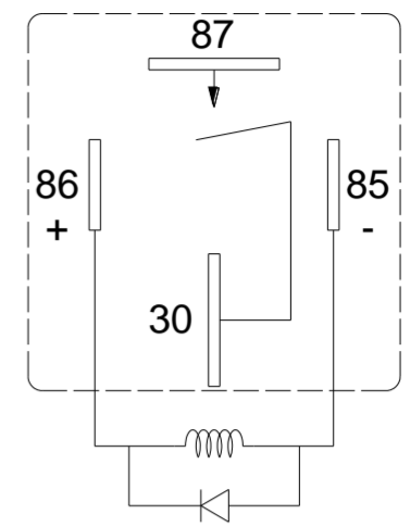
With Parallel Diode (Anode on 85#)
